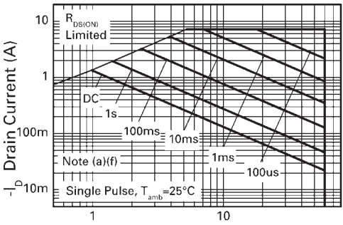
-V_{DS} Drain-Source Voltage (V) P-channel Safe Operating Area
