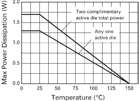
Derating Curve
