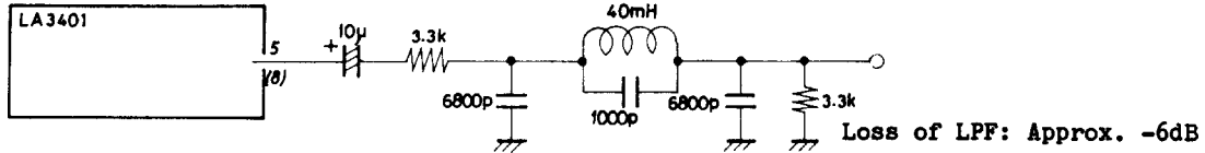
Fig. 16 Sample LC filter circuit (including de-emphasis circuit)
