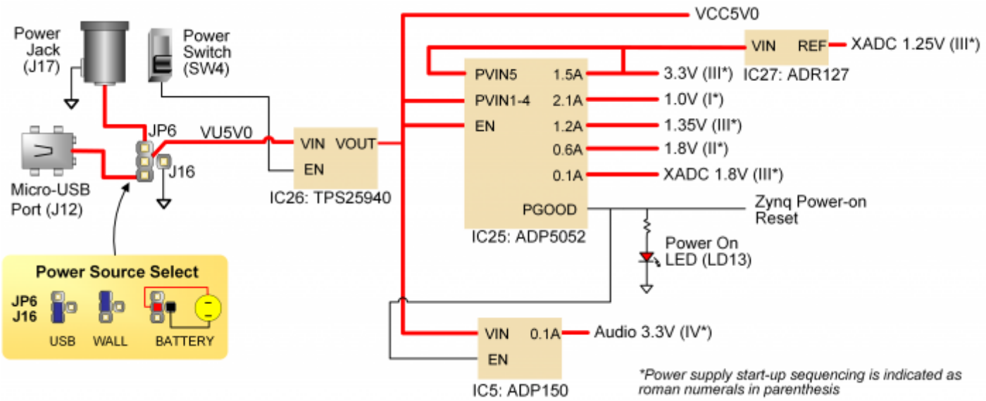
Figure 1.1. Power circuit overview
