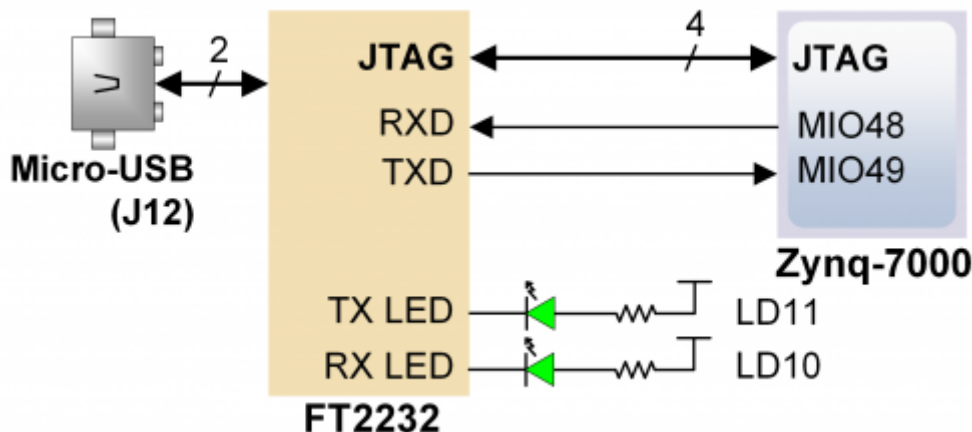
Figure 7.1. UART Connections
