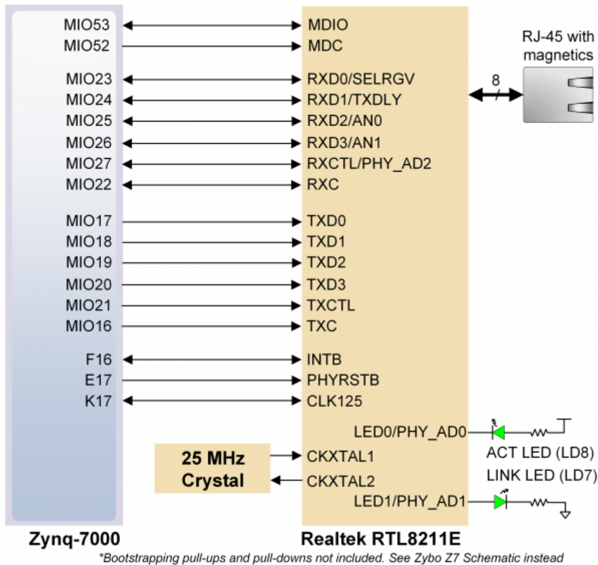
Figure 10.1. Ethernet PHY signals
