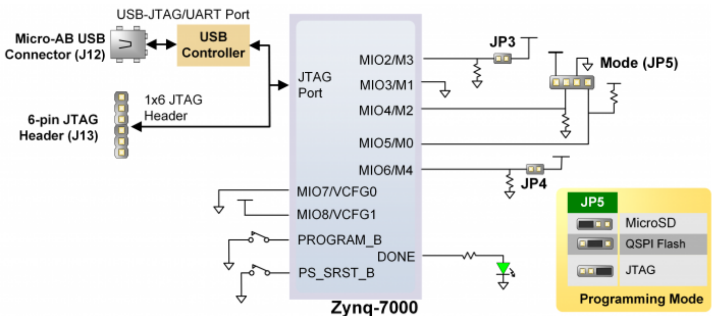
Figure 2.1. Zybo Z7 configuration pins.
