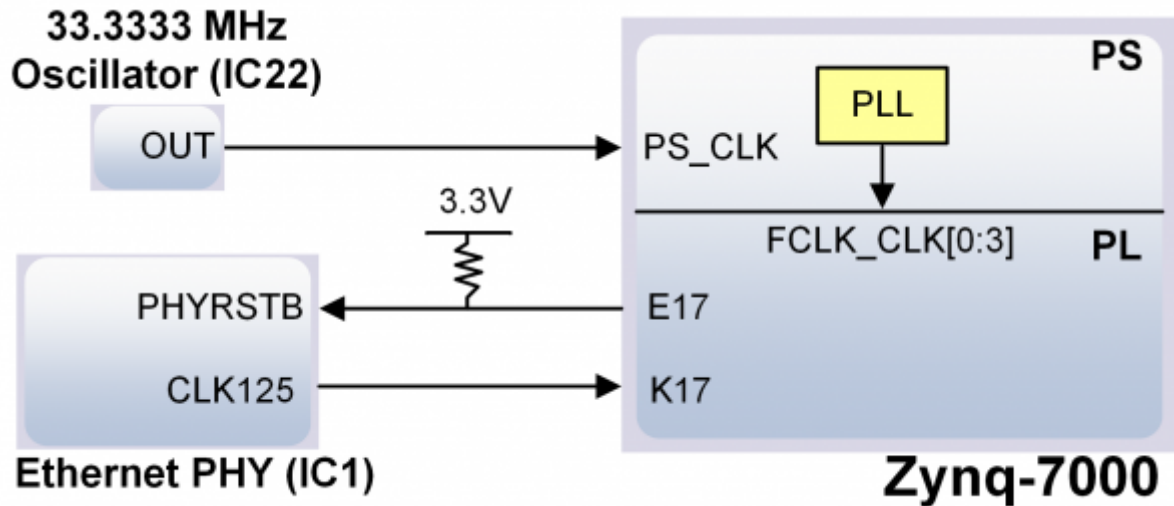
Figure 5.1. Zybo Z7 clocking.
