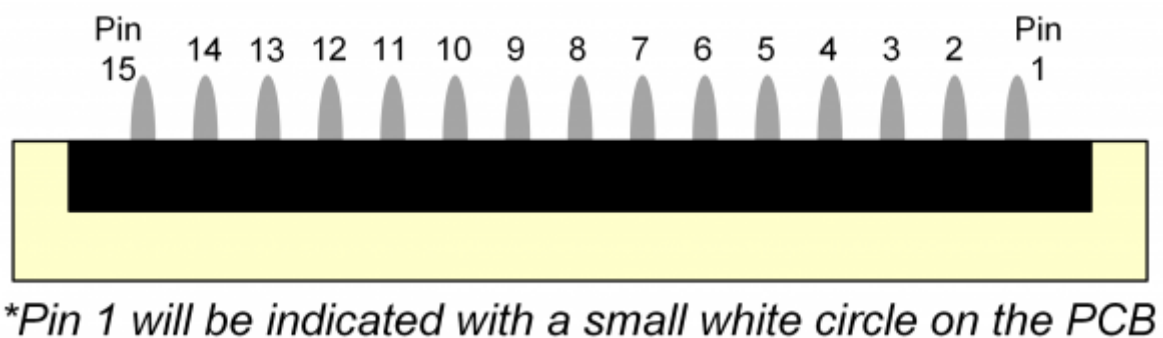
Figure 15.1. Pcam Pin-out
