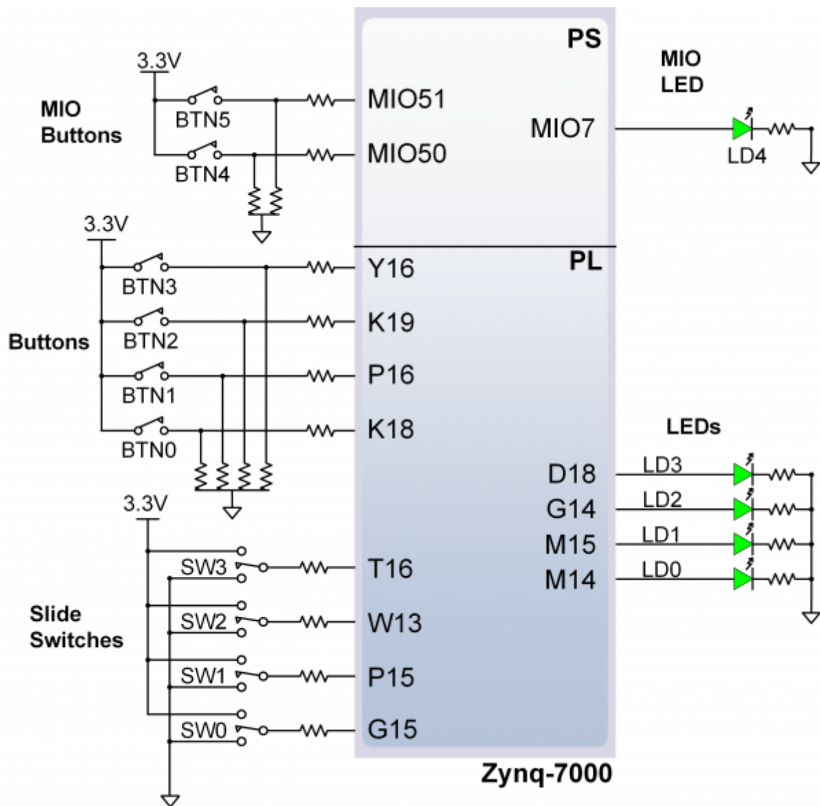
Figure 13.1. Zybo Z7 GPIO
