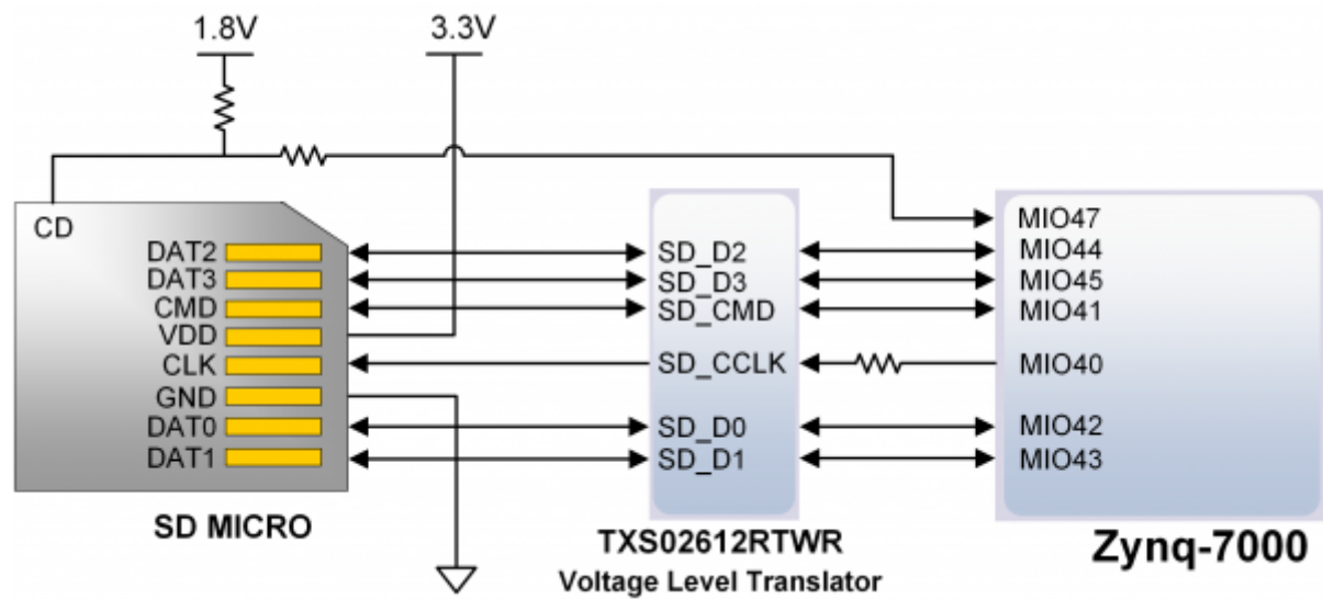
Figure 8.1. microSD slot signals
