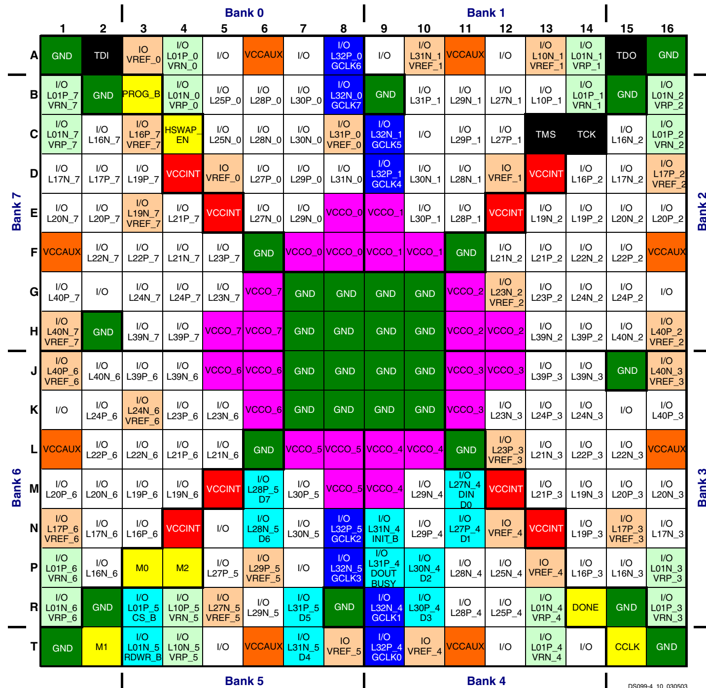
Figure 12: FT256 Package Footprint (top view)
