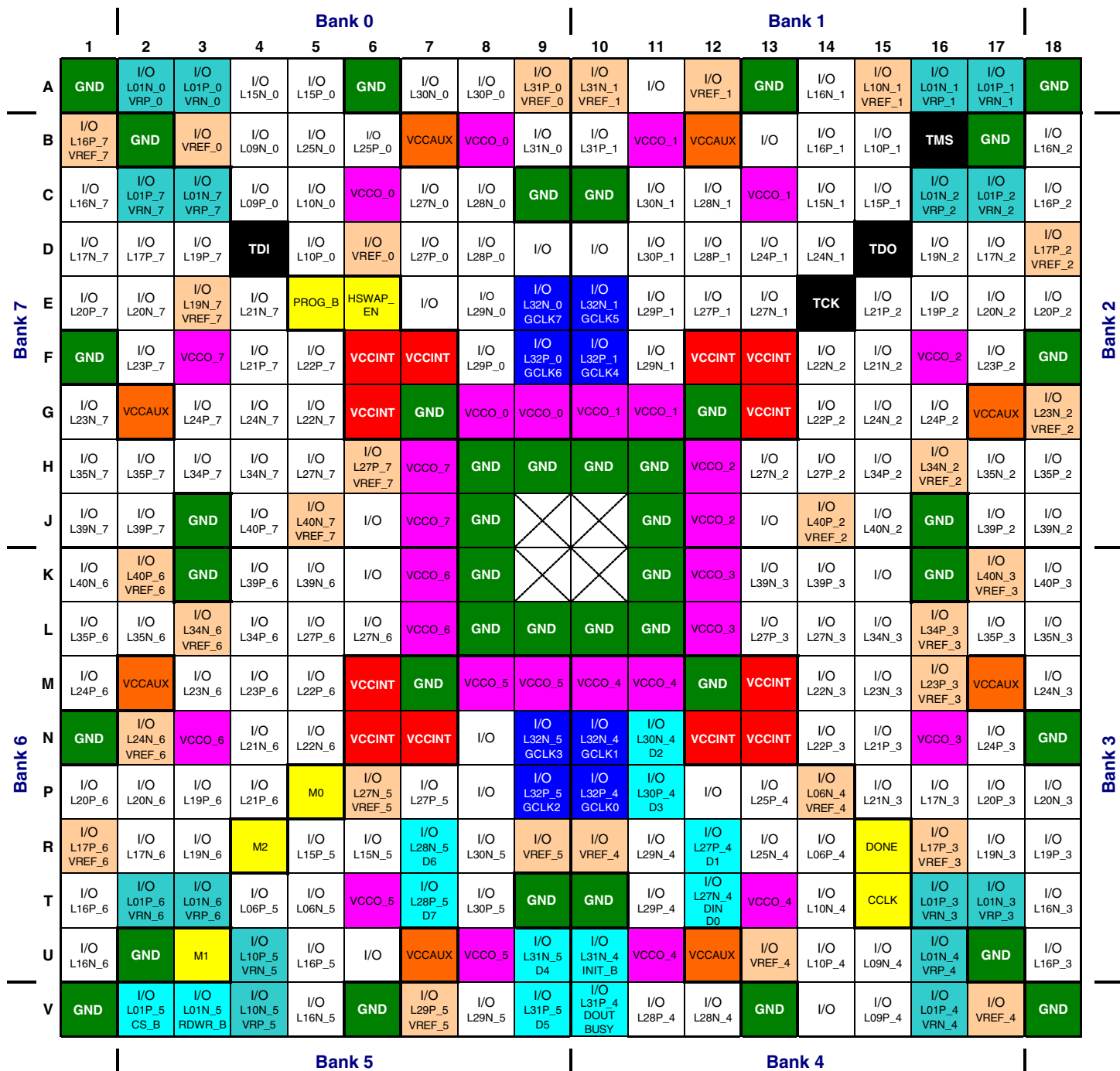
Figure 13: FG320 Package Footprint (top view)
