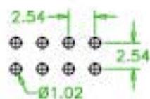
Recommended P.C.B Hole Layout
