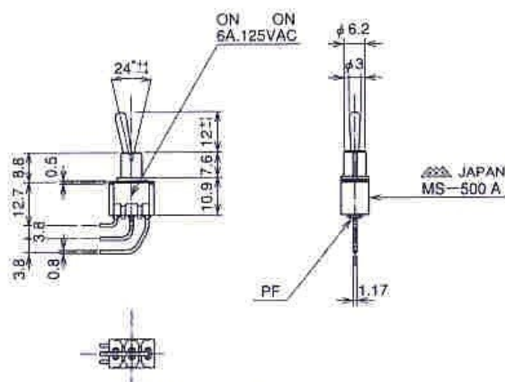
(3P) MS-500A-B-VT
