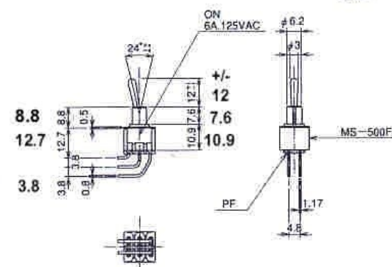
(6P) MS-500F-B-VT
